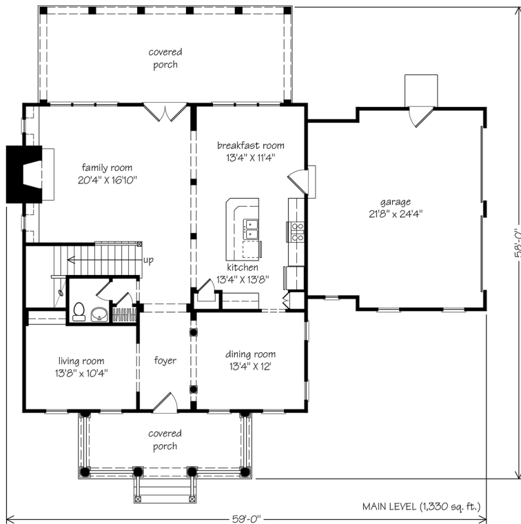
#1680 Old Ivy: Main Level Floor Plan
