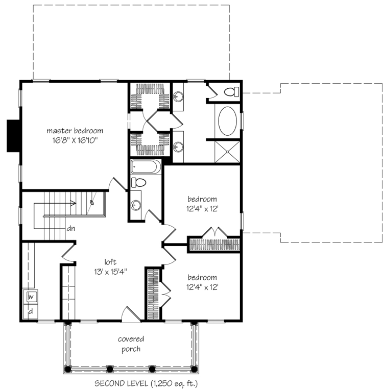
#1680 Old Ivy: Second Level Floor Plan
